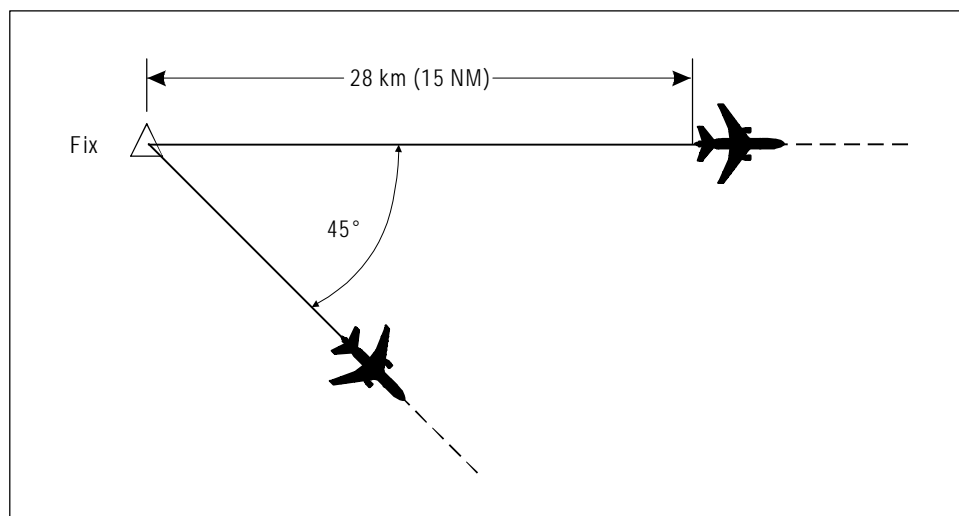
Figure 5-4. Separation using dead reckoning (see 5.4.1.2.1.2 c))
