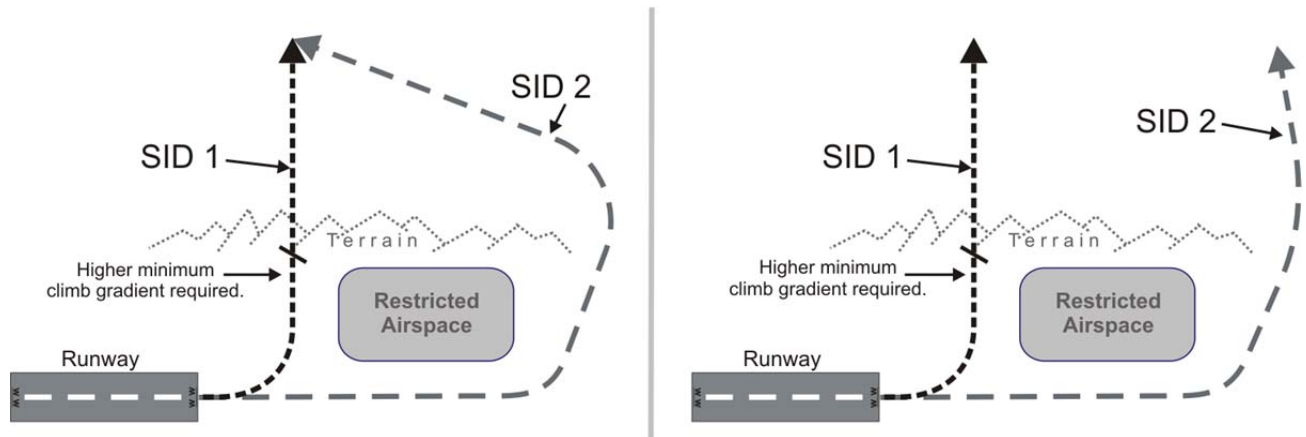
Figure 1.3. Multiple CCO SID Design – Top View
