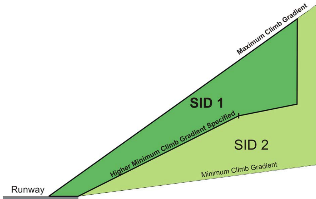
Figure 1.2. Multiple CCO SID Design – Profile View
