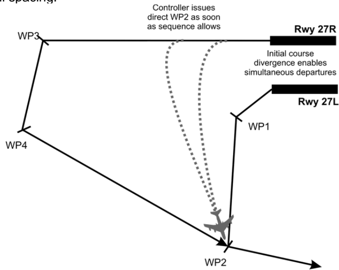
Figure 1.5. Multiple Runway CCO SID Design
