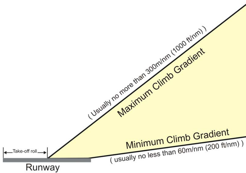
Figure 1.1. Basic CCO
