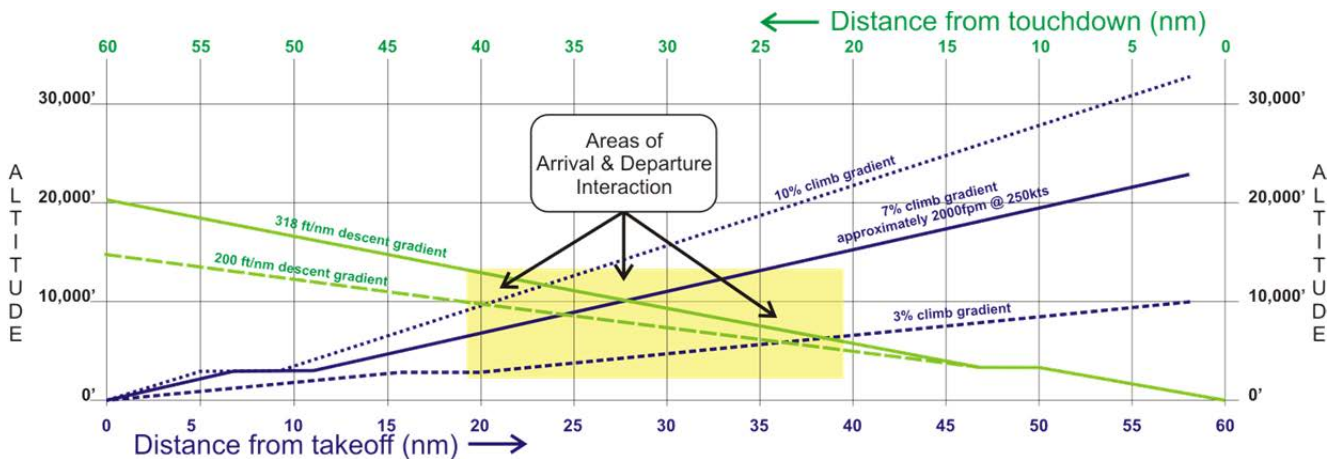
Figure 2.1 Possible Vertical Interaction Between Departing and Arriving Traffic
