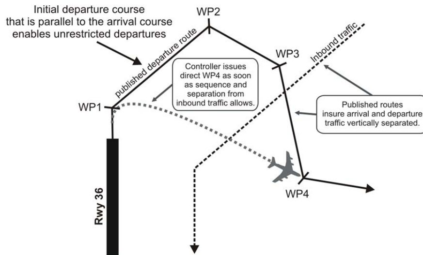
Figure 1.4. CCO SID Parallel to Arrival
